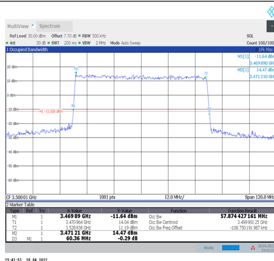
1-N78-3450-3550--30-60-M-1-DFT-QPSK-Outer_Full-162@0-Ant1-57.874-60.360-≤60-PASS
