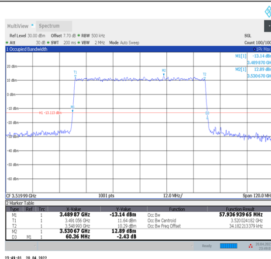
1-N78-3450-3550--30-60-H-4-DFT-64QAM-Outer_Full-162@0-Ant1-57.937-60.360-≤60-PASS
