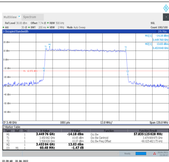
1-N78-3450-3550--30-60-L-7-CP-16QAM-Outer_Full-162@0-Ant1-57.835-60.480-≤60-PASS
