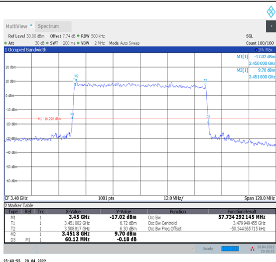
1-N78-3450-3550--30-60-L-9-CP-256QAM-Outer_Full-162@0-Ant1-57.734-60.120-≤60-PASS
