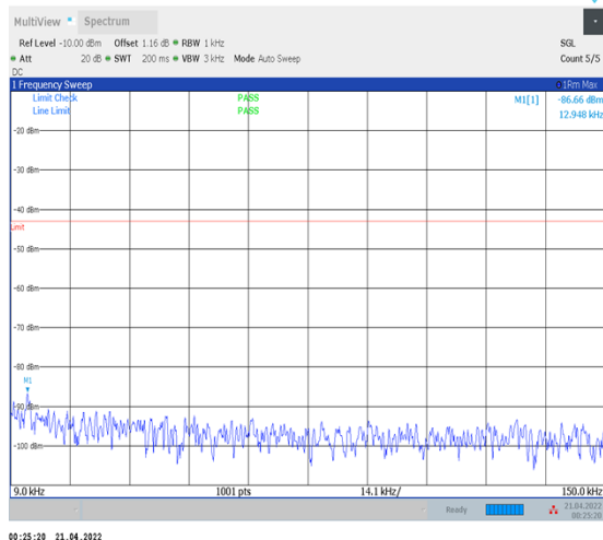
1-N78-3450-3550--30-100-H-1-DFT-PI2BPSK- Inner_1RB_Left-1@1-0.009-0.15-Ant1--86.66--43- PASS
