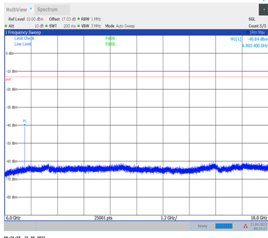
1-N78-3450-3550--30-100-L-1-DFT-PI2BPSK- Inner_1RB_Left-1@1-6000-18000-Ant1--40.84--13- PASS
