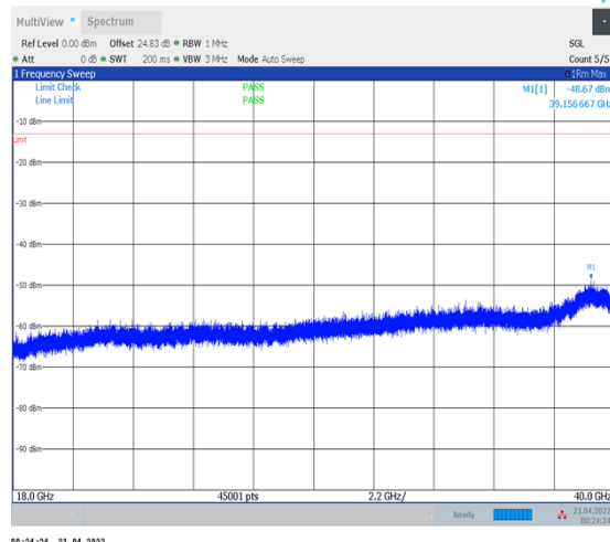
1-N78-3450-3550--30-100-L-1-DFT-PI2BPSK- Inner_1RB_Left-1@1-18000-40000-Ant1--48.67--13- PASS
