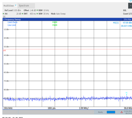
1-N78-3450-3550--30-100-M-1-DFT-PI2BPSK- Inner_1RB_Left-1@1-0.15-30-Ant1--87.00--33-PASS
