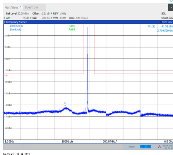
1-N78-3450-3550--30-100-H-1-DFT-PI2BPSK- Inner_1RB_Left-1@1-1000-6000-Ant1--41.52--13- PASS
