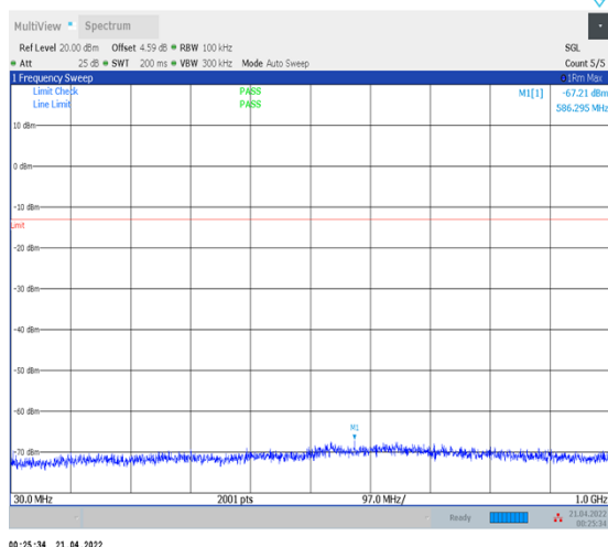
1-N78-3450-3550--30-100-H-1-DFT-PI2BPSK- Inner_1RB_Left-1@1-30-1000-Ant1--67.21--13- PASS
