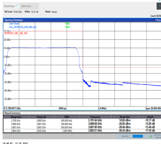
1-N78-3700-3800-PC2-30-10-H-6-CP-QPSK-Outer_Full-24@0-Ant1-PASS-see graph
