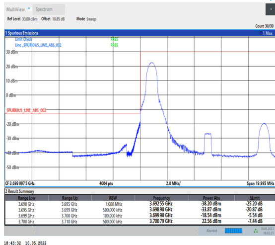
1-N78-3700-3800-PC2-30-10-L-4-CP-QPSK-Edge_1RB_Left-1@0-Ant1-PASS-see graph
