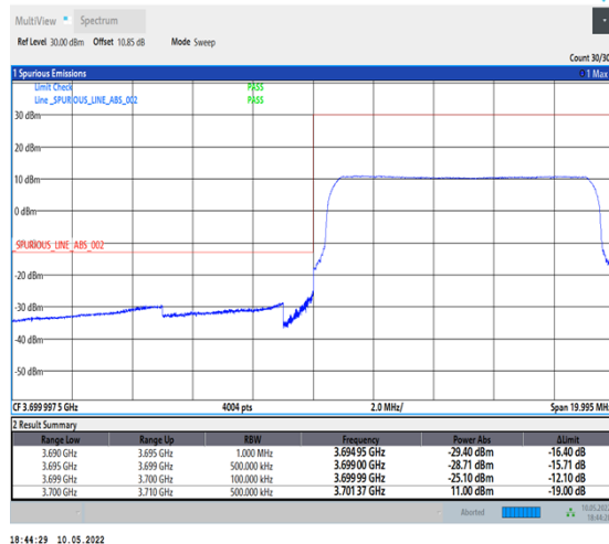
1-N78-3700-3800-PC2-30-10-L-6-CP-QPSK-Outer_Full-24@0-Ant1-PASS-see graph
