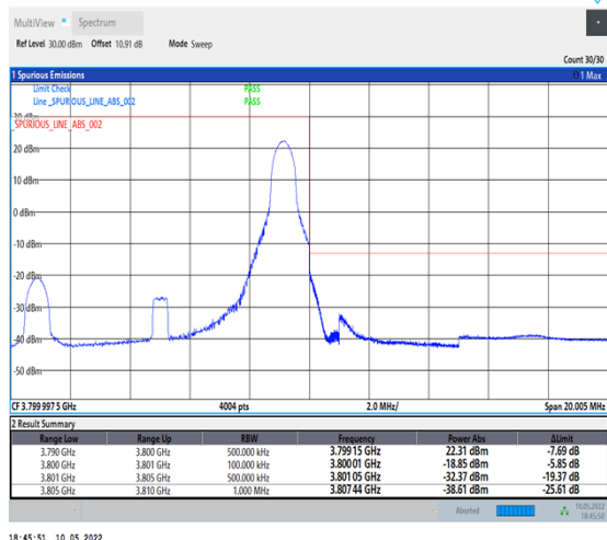
1-N78-3700-3800-PC2-30-10-H-5-CP-QPSK-Edge_1RB_Right-1@23-Ant1-PASS-see graph
