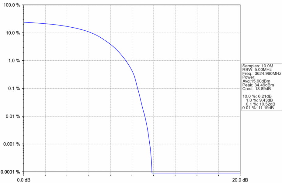
n48_30kHz_SISO_NTNV_10MHz_DFT-s-OFDM QPSK_3624.99MHz_Outer_Full
