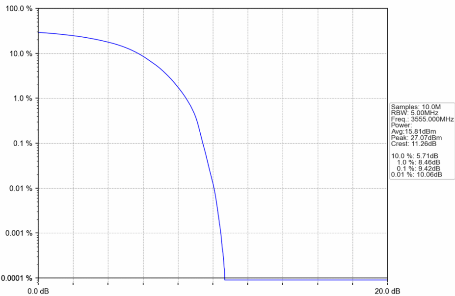
n48_30kHz_SISO_NTNV_10MHz_DFT-s-OFDM QPSK_3555MHz_Outer_Full
