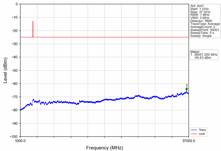
n48_30kHz_SISO_NTNV_20MHz_CP-OFDM_QPSK_3690MHz_Edge_1RB_Right
