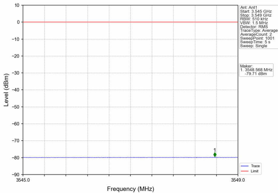
n48_30kHz_SISO_NTNV_40MHz_DFT-s-OFDM QPSK_3570MHz_Outer_Full
