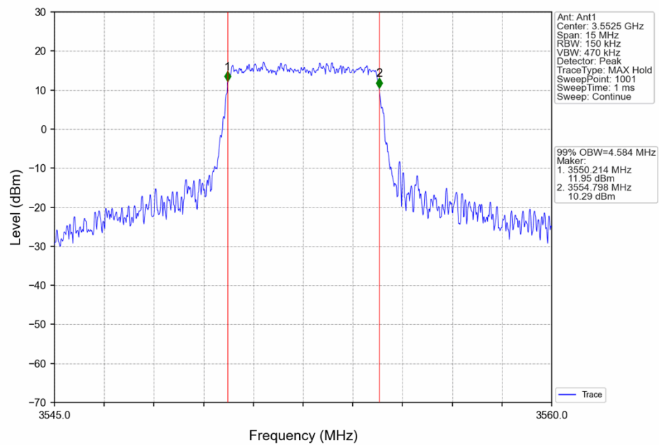
Band48_5MHz_16QAM_LCH_3552.5MHz_RB_25_0_NTNV
