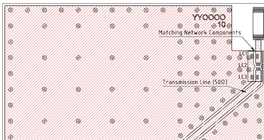
Matching network drawing (LC1=0.3pF, LC2=1.0nH, LC3=0.3pF)
