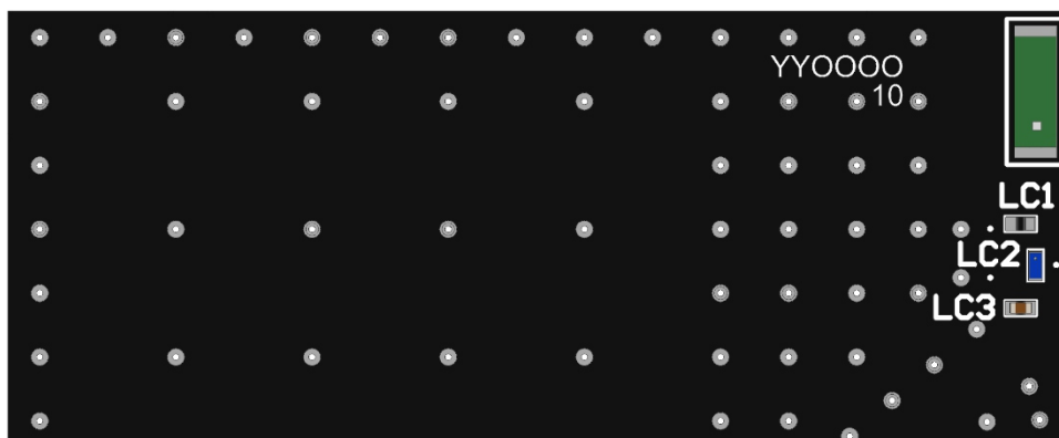
3D View of matching components and recommended values (LC1 = 0.3pF, LC2=1.0nH, LC3= 0.3pF)
