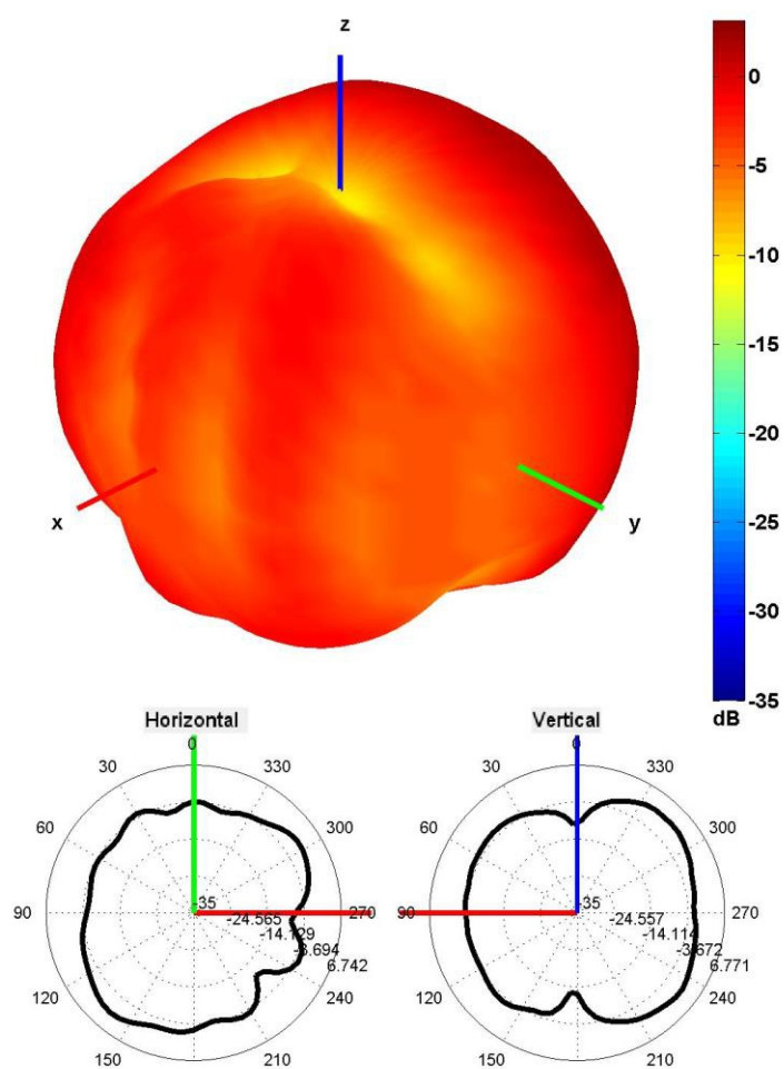
5500 MHz Radiation pattern
