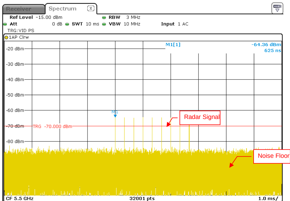
Radar Signal 6
