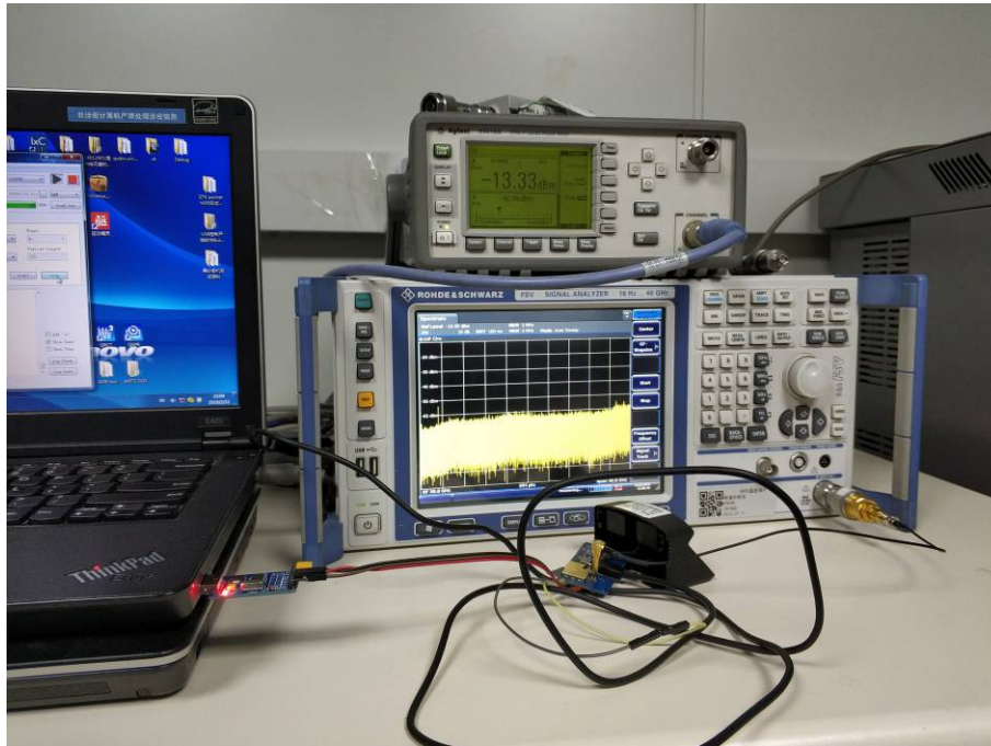
RF Conducted Test setup (BLE/WIFI)
