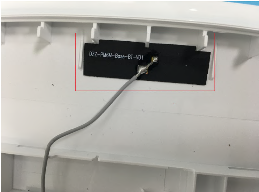
BT antenna
