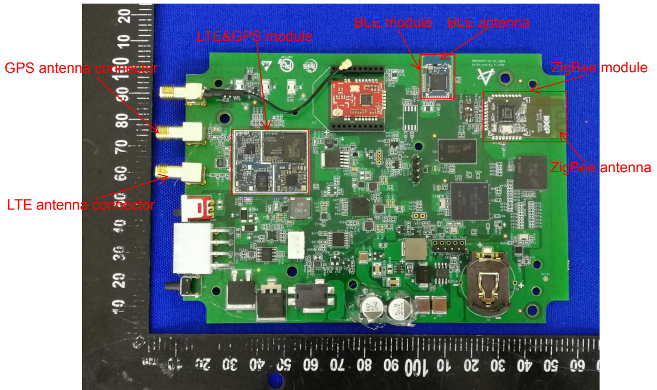
MAIN BOARD TOP VIEW (WITHOUT SHIELDING)
