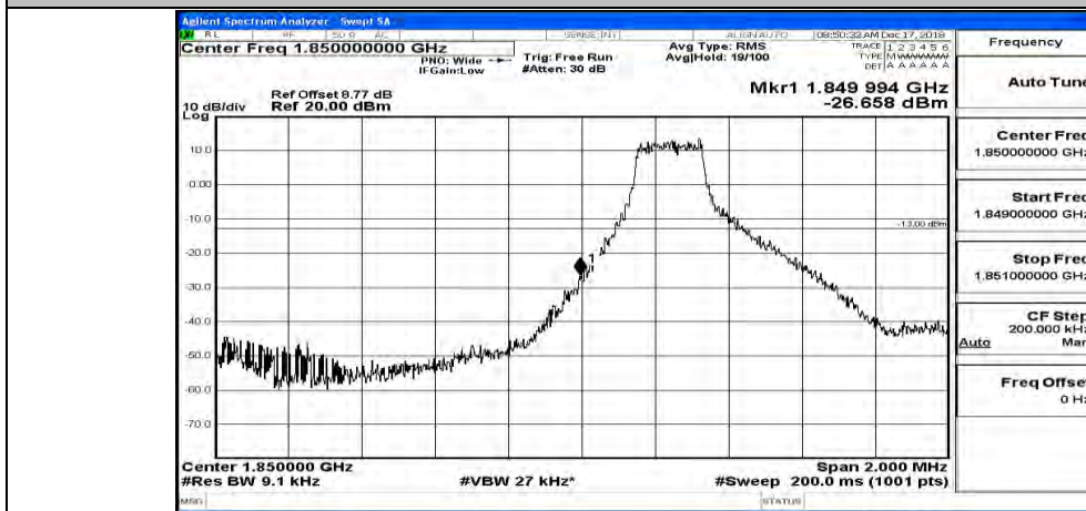
(Channel Bandwidth: 3 MHz)_LCH_QPSK_1RB#7
