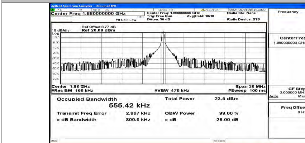
(Channel Bandwidth:15 MHz)_MCH_QPSK_1RB#74
