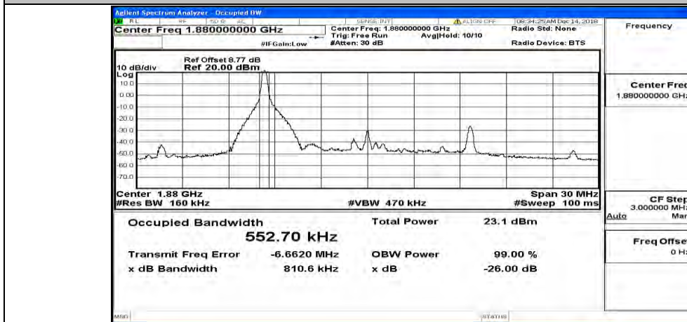
(Channel Bandwidth:15 MHz)_MCH_QPSK_1RB#37
