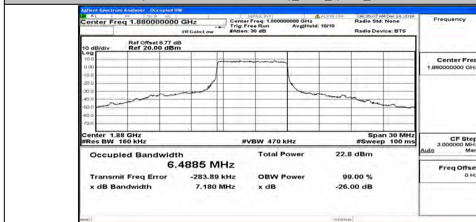
(Channel Bandwidth:15 MHz)_MCH_QPSK_37RB#38
