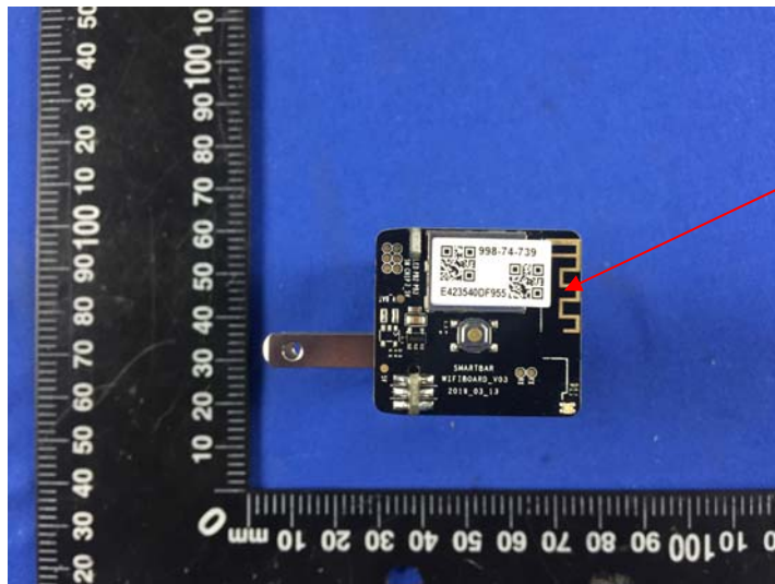
WIFI Antenna
