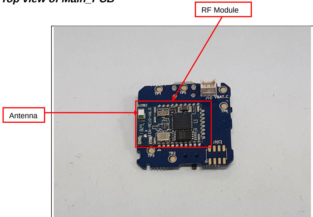
Top view of Main_PCB
