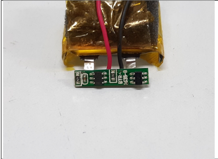
Bottom view of Sub_PCB2
