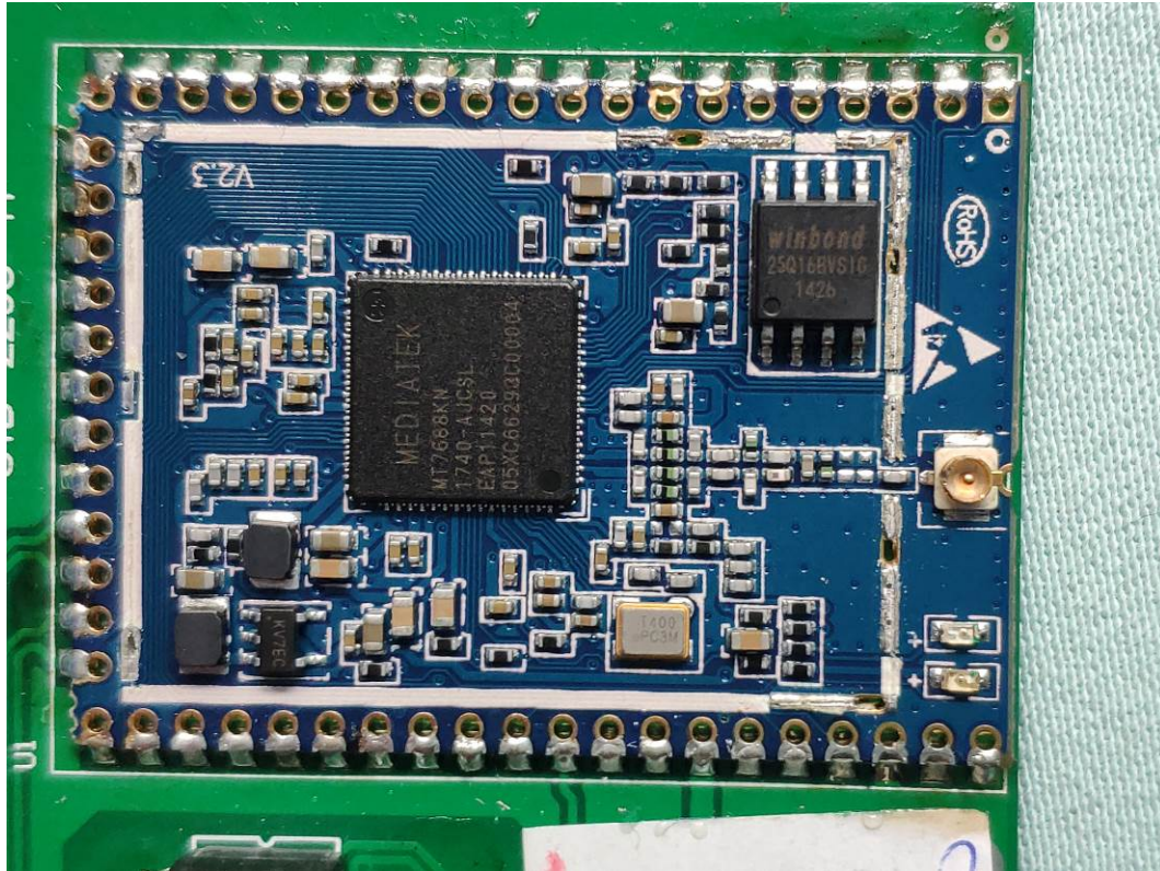
FIGURE 7 WIRELESS ETHERNET BRIDGE (M/N: WB-10) CHIP & CRYSTAL ON MAIN BOARD
