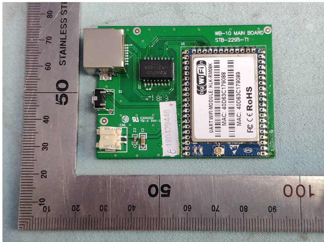
FIGURE 5 WIRELESS ETHERNET BRIDGE (M/N: WB-10) MAIN BOARD (COMPONENT SIDE)
