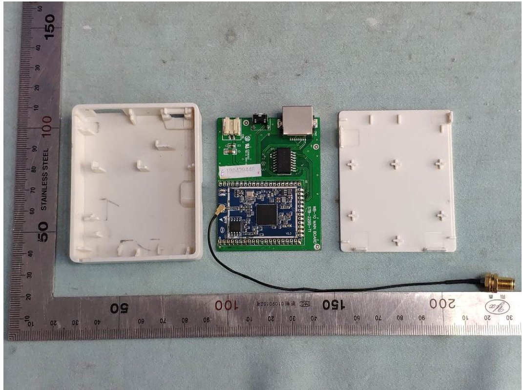
FIGURE 4 WIRELESS ETHERNET BRIDGE (M/N: WB-10) COVER REMOVED
