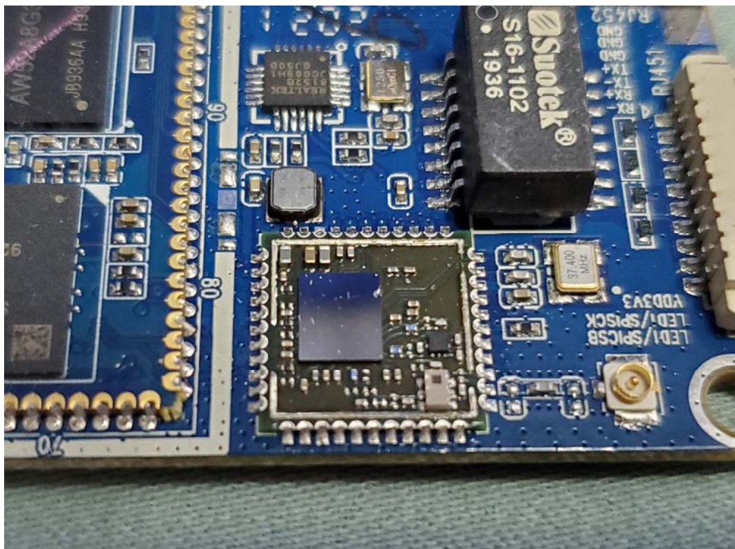
FIGURE 11 SMART CARD TERMINAL (M/N: WB-20) CRYSTAL & CHIP ON MAIN BAORD
