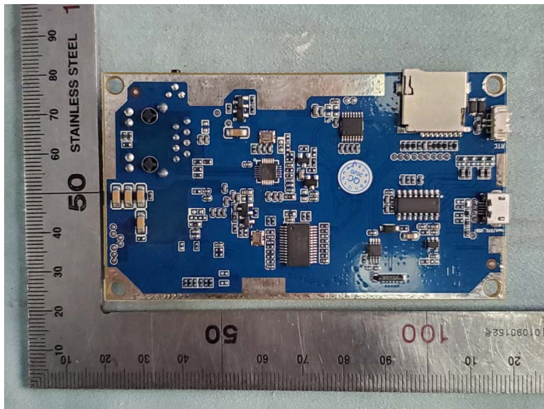
FIGURE 9 SMART CARD TERMINAL (M/N: WB-20) MAIN BOARD (SOLDERED SIDE)
