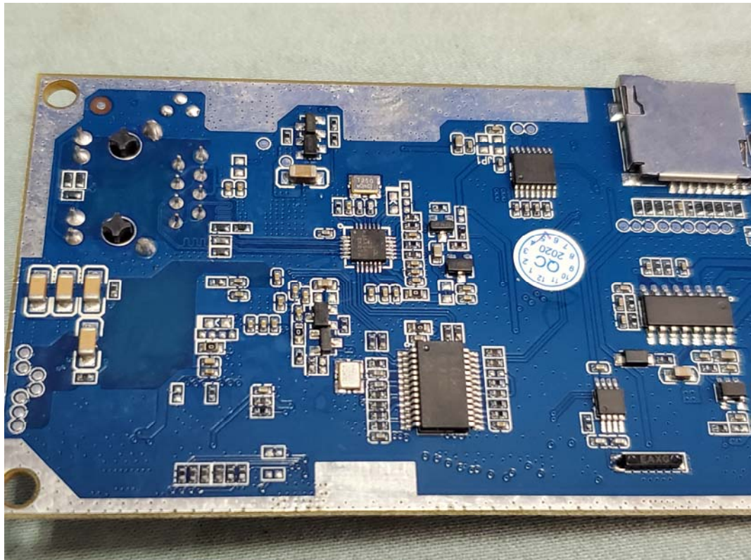
FIGURE 12 SMART CARD TERMINAL (M/N: WB-20) CRYSTAL & CHIP ON MAIN BAORD
