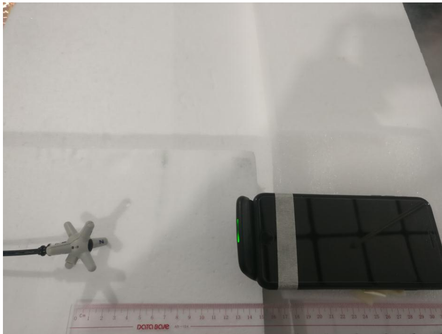
E-field Test Setup Photo Positon C(15mm)
