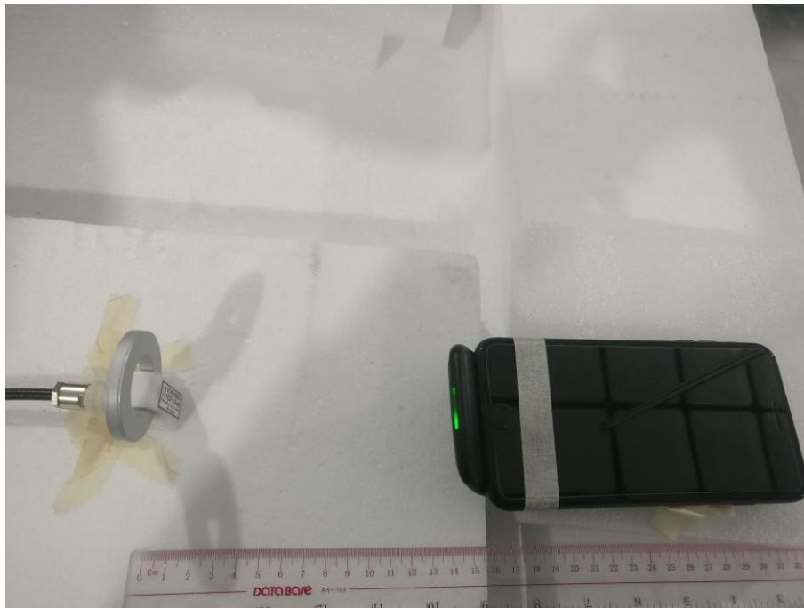
H-field Test Setup Photo Positon C(15mm)
