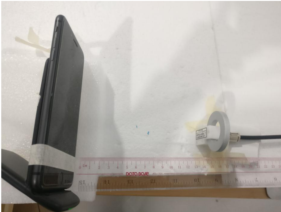
H-field Test Setup Photo Positon E(15mm)
