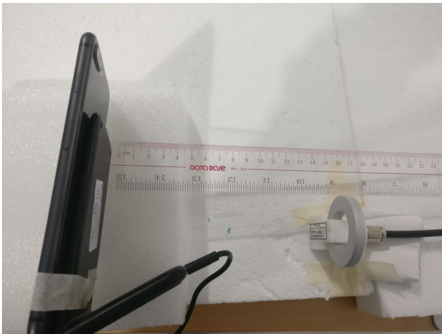
H-field Test Setup Photo Positon F(15mm)
