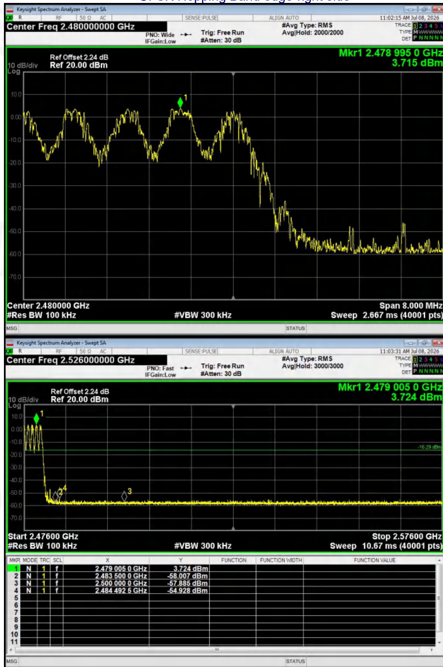
GFSK Hopping Band edge-right side
