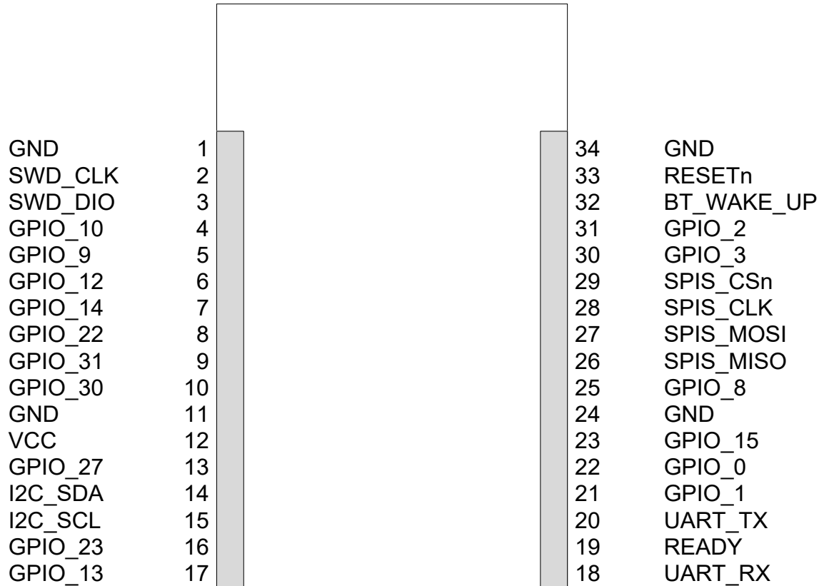
Figure 1: DWM1001C Pin Diagram
