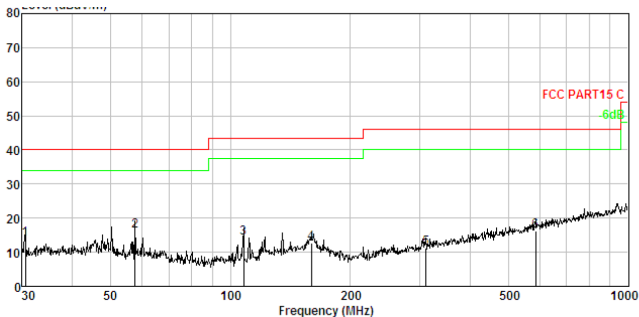
Test plot for Vertical: GFSK(2402MHz)
