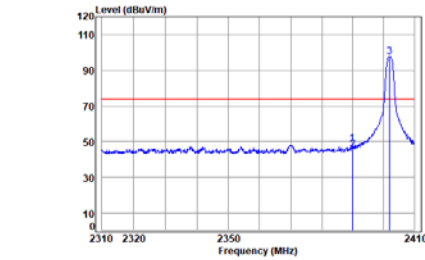
BLE_1M_TX_CH_00_Horizontal-Peak
