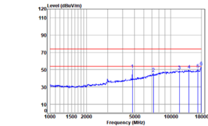
BLE_2M_TX_CH_00_Horizontal
