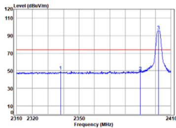
BLE_2M_TX_CH_00_Vertical-Peak
