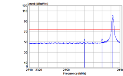
BLE_1M_TX_CH_00_Vertical-Peak
