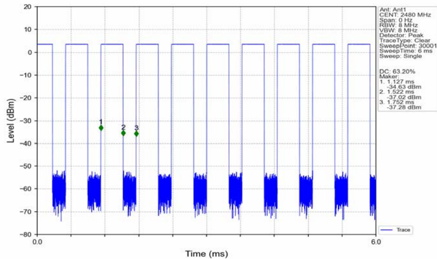
1M_HCH_2480MHz_Ant1_NTNV
