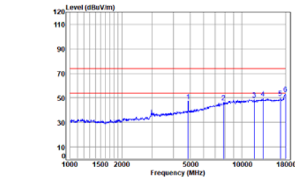
BLE_2M_TX_CH_19_Horizontal
