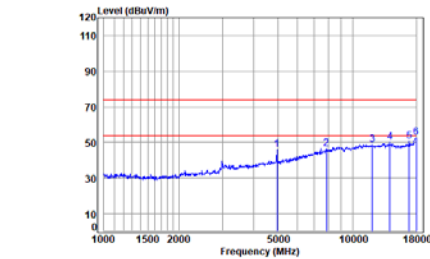
BLE_1M_TX_CH_39_Horizontal
