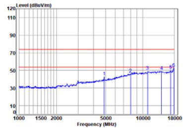
BLE_2M_TX_CH_19_Vertical
