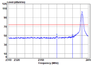
BLE_2M_TX_CH_00_Horizontal-Peak
