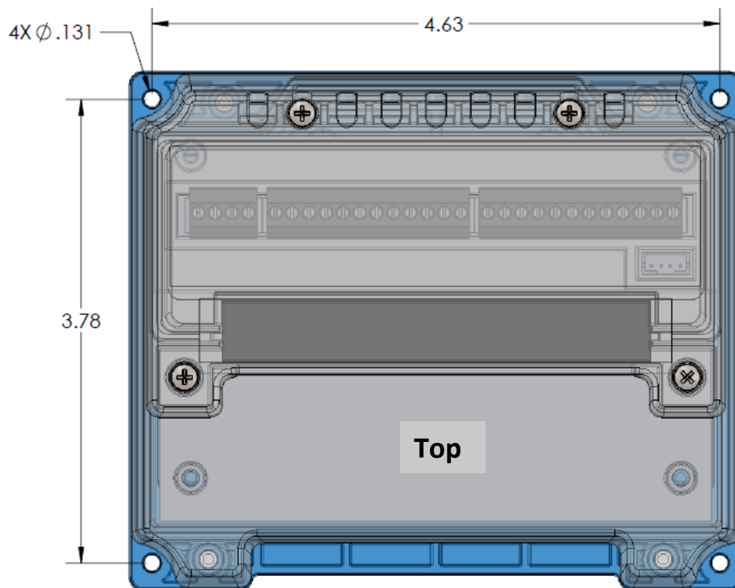
MOUNTING DIMENSIONS
