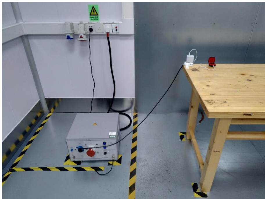
Conducted Emission For AC Mains Power Ports
