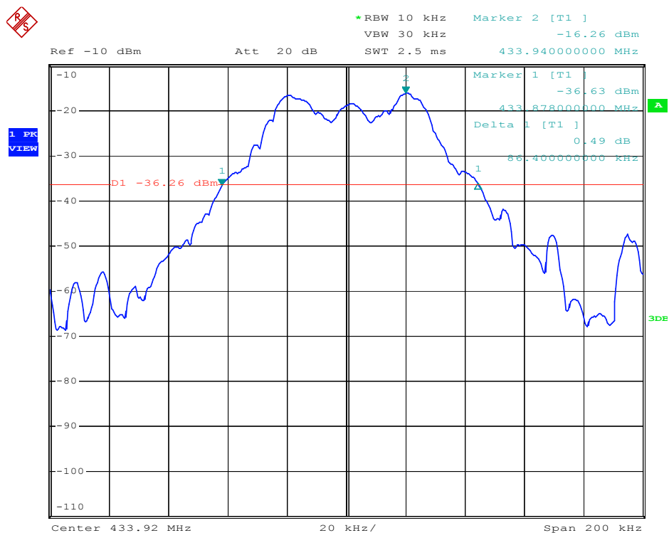
20dB Bandwidth Test Plot
