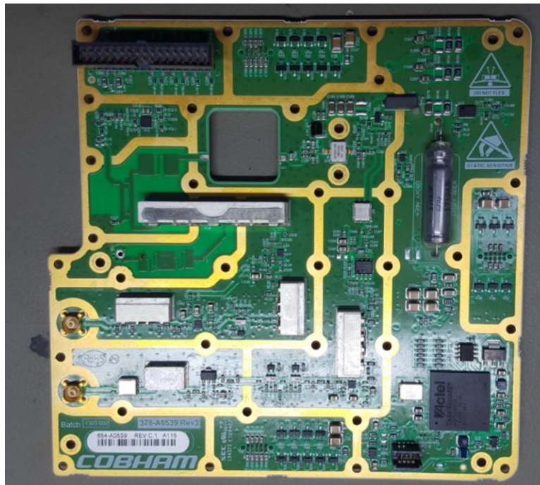
Figure 3: RF Board (Top)
