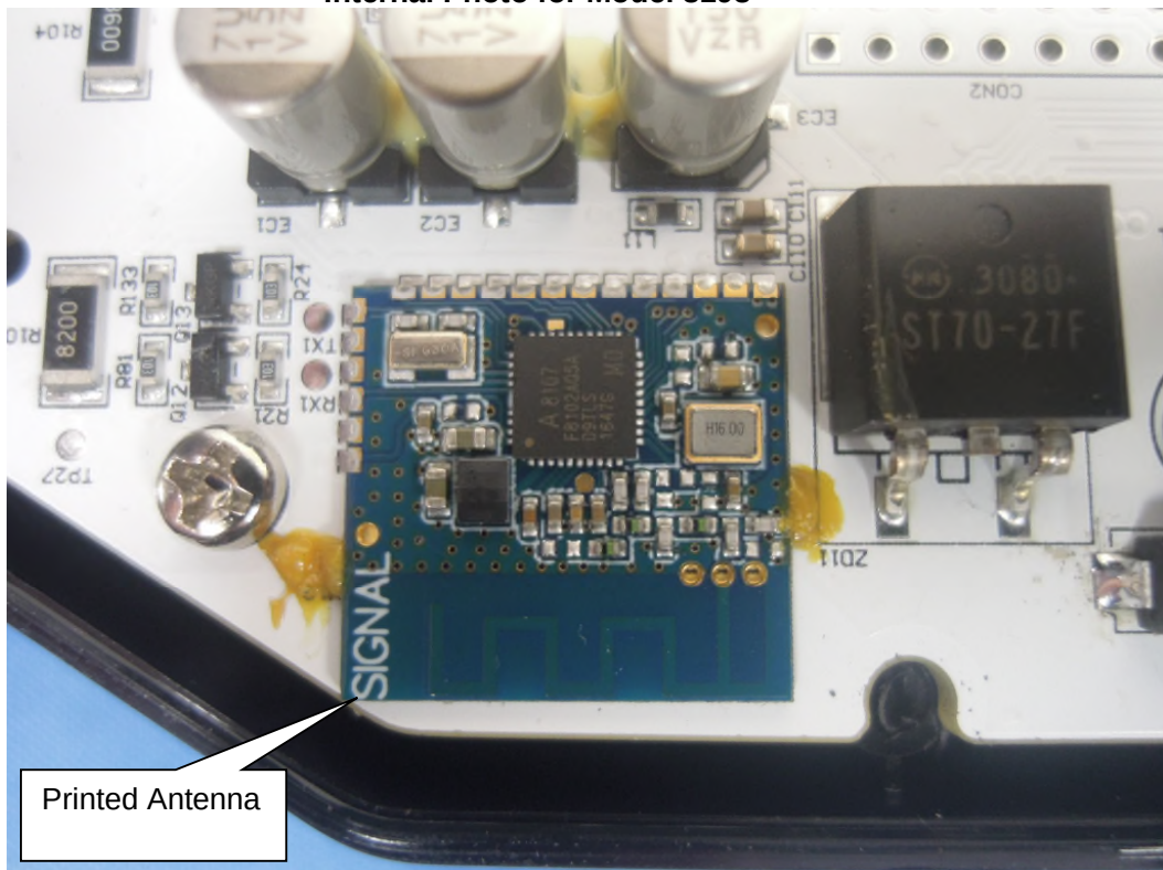
Internal Photo for Model 8198
