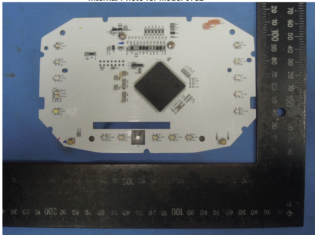
Internal Photo for Model 0782
