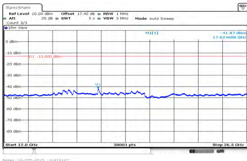
Band4-10MHz-16QAM-20350-1RB#0-Range4:12000~26500MHz
