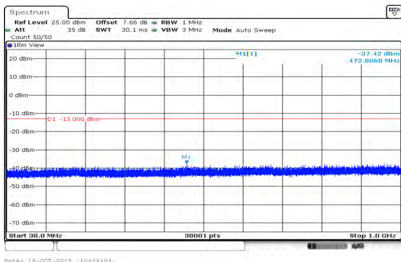
Band4-3MHz-16QAM-20175-1RB#0-Range1:30~1000MHz
