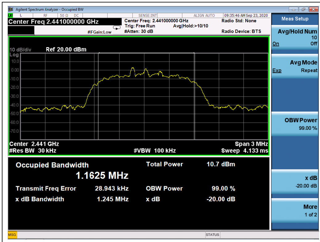
(Channel 39, 8-DPSK)
