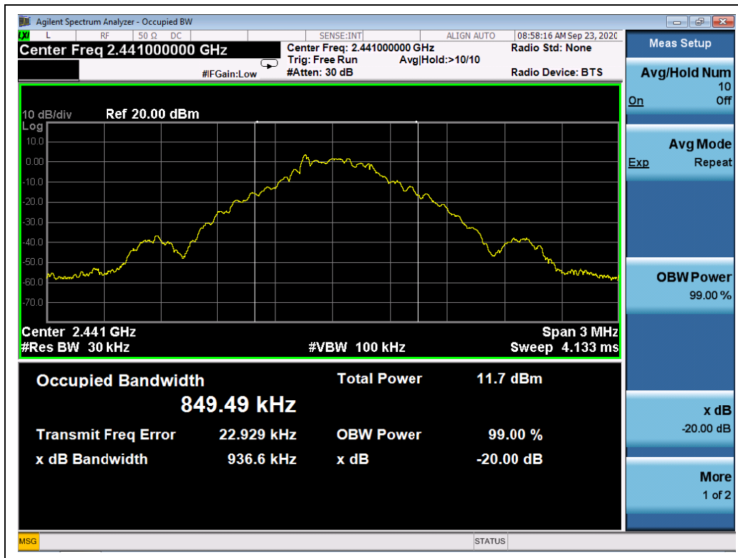
(Channel 39, GFSK)
