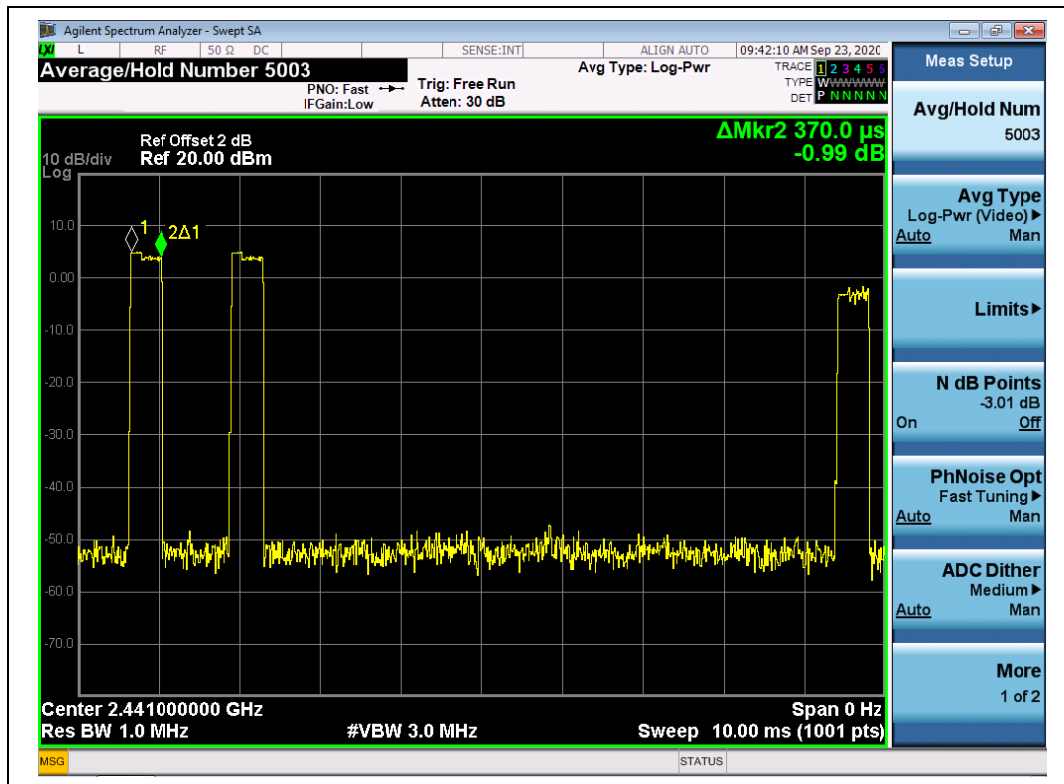
(DH1, π/4-DQPSK)
