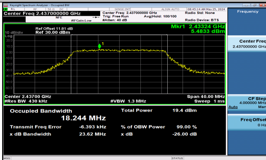
11N20SISO-Ant1-2437
