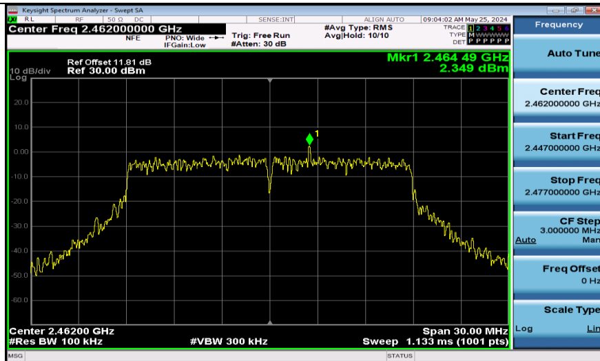
11N20SISO-Ant1-2462-0~Reference-PASS
