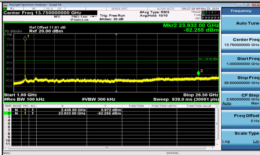
11B-Ant1-2437-1000~26500-PASS
