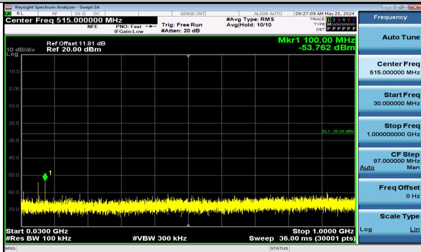
11B-Ant1-2437-30~1000-PASS
