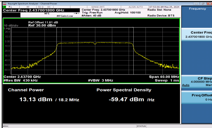
11N20ISO-Ant1-2437-PASS
