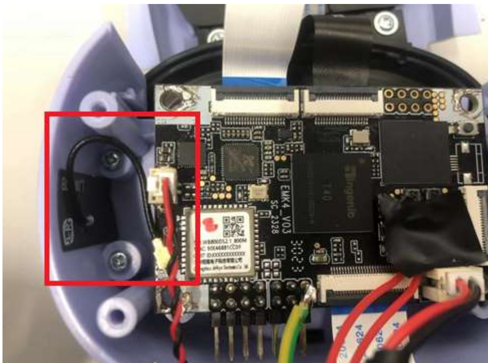
Location of antenna (Internally)
