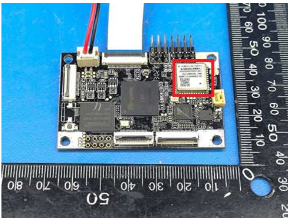
PCB view (WIFI module)
