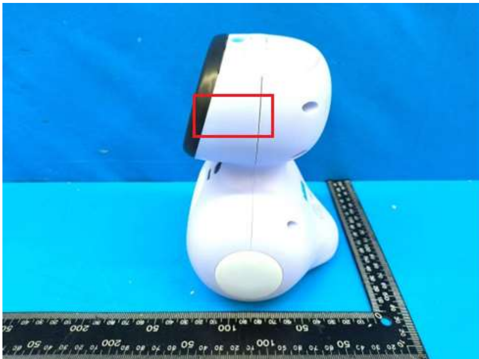
Location of antenna (Externally)
