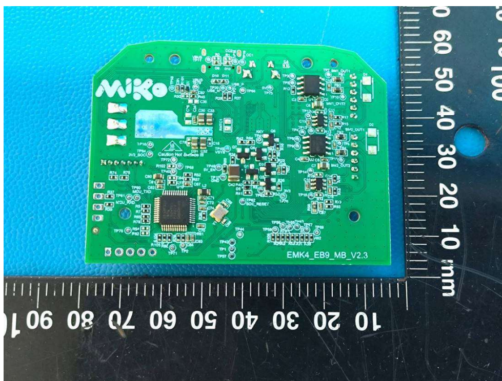
PCB view
