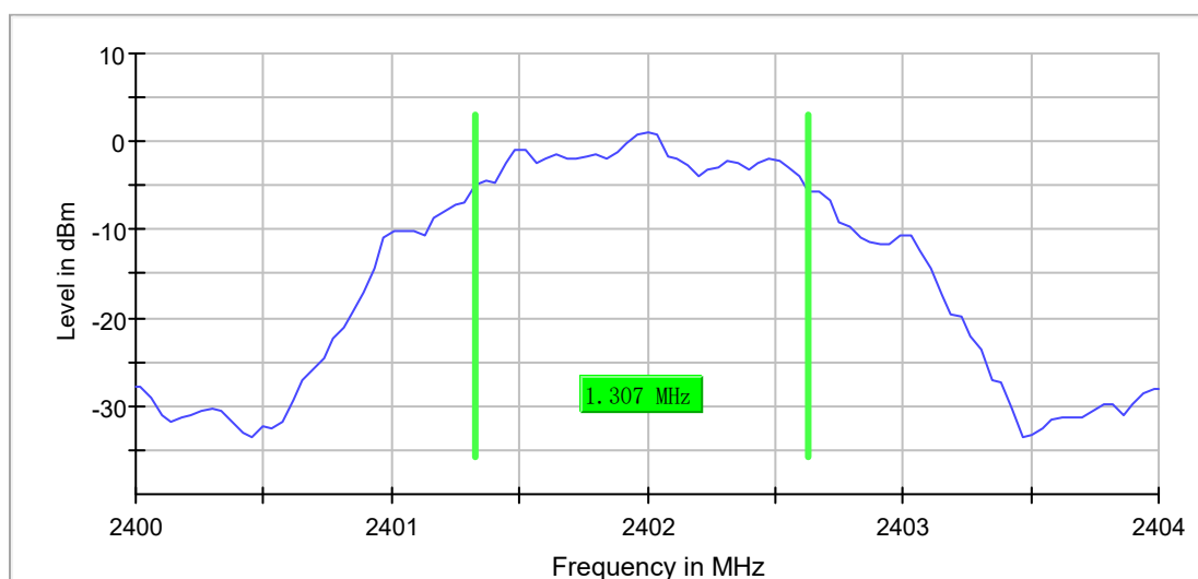
6dB Occupied Bandwidth Mode 2 / CH0 (2402 MHz)
