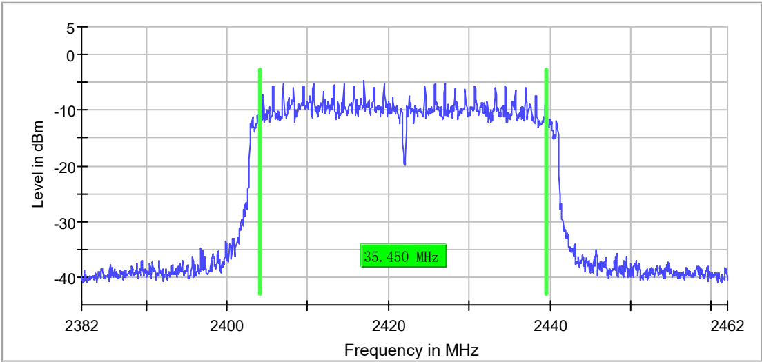
6dB Occupied Bandwidth Mode 1 / CH2 (2422MHz)
