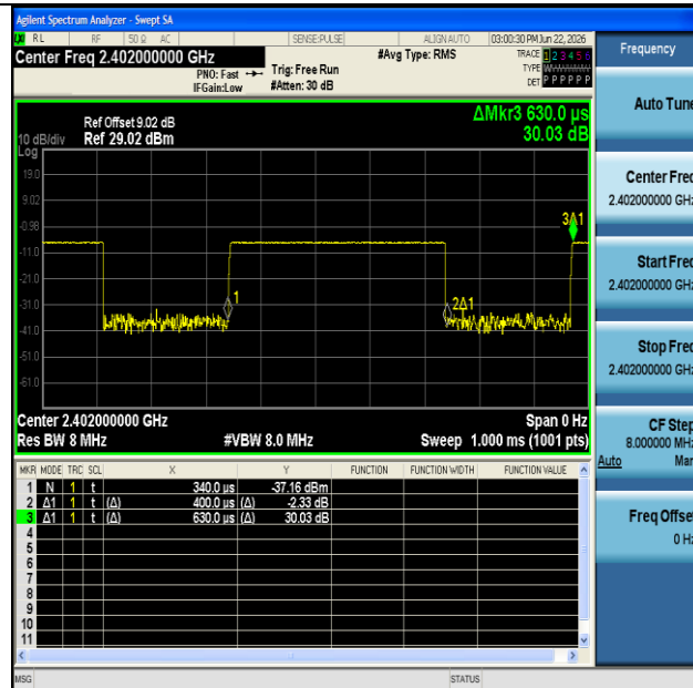
NTNV-BLE_1M-Ant1-2402
