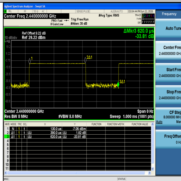
NTNV-BLE_1M-Ant1-2440
