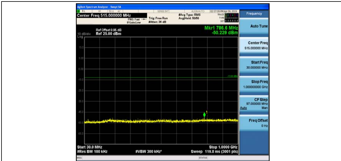
Band4_1.4MHz_QPSK_20393_1RB#0
