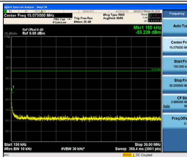
Band5_1.4MHz_16QAM_20643_1RB#0
