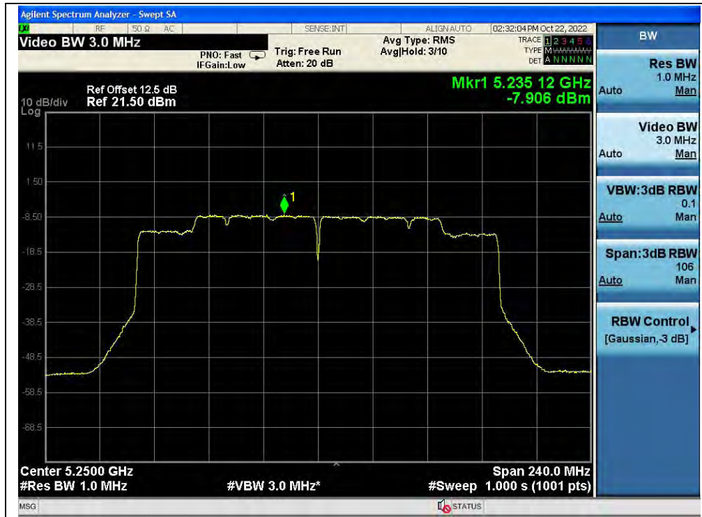
(Channel 50, 5250MHz, 802.11ax (HEW160), ANT0)
