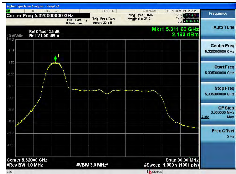
(Channel 64, 5320MHz, 802.11ax (HEW20) RU26, ANT0)
