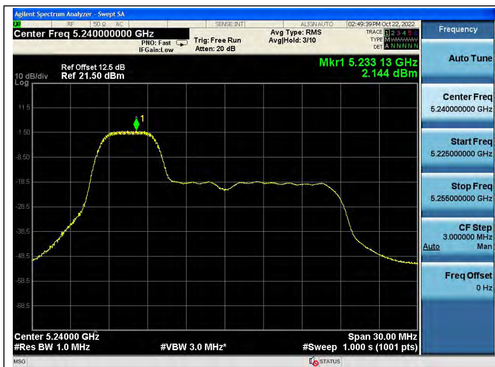
(Channel 48, 5240MHz, 802.11ax (HEW20) RU52, ANT0)
