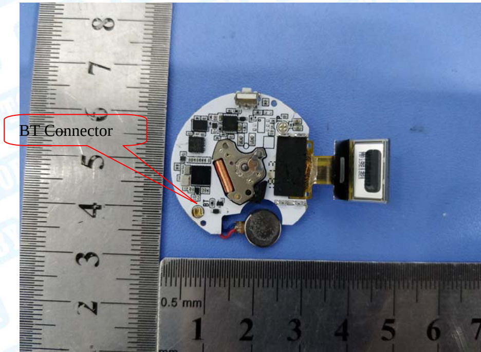
Photo 10 Appearance of PCB
