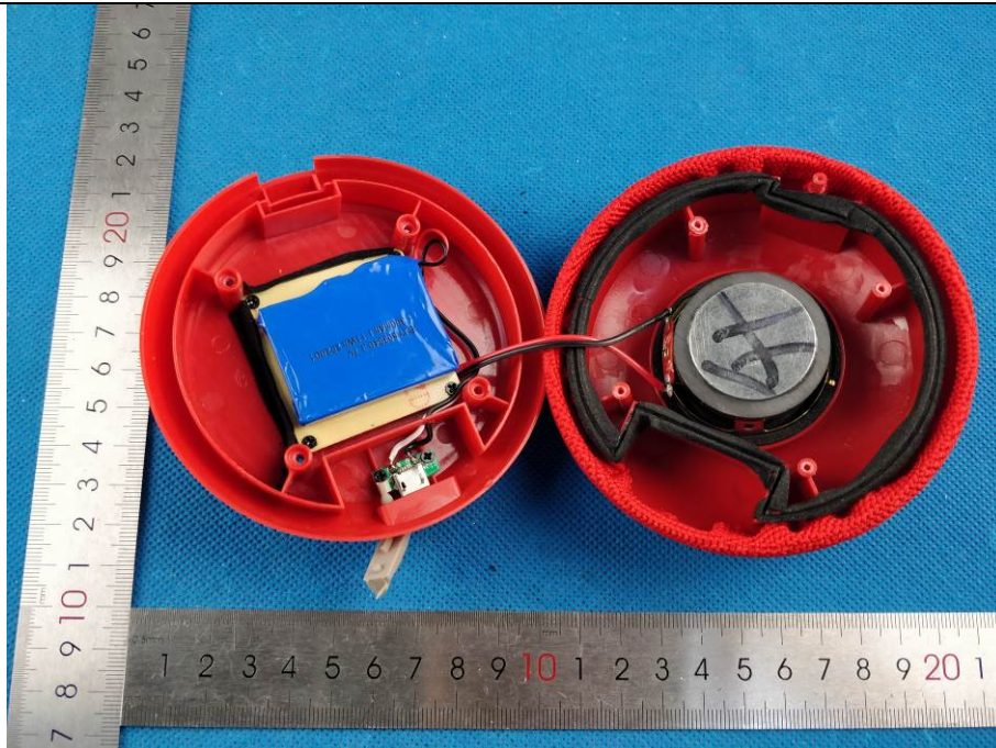
Photo 1 (For model EBT-1008B)
