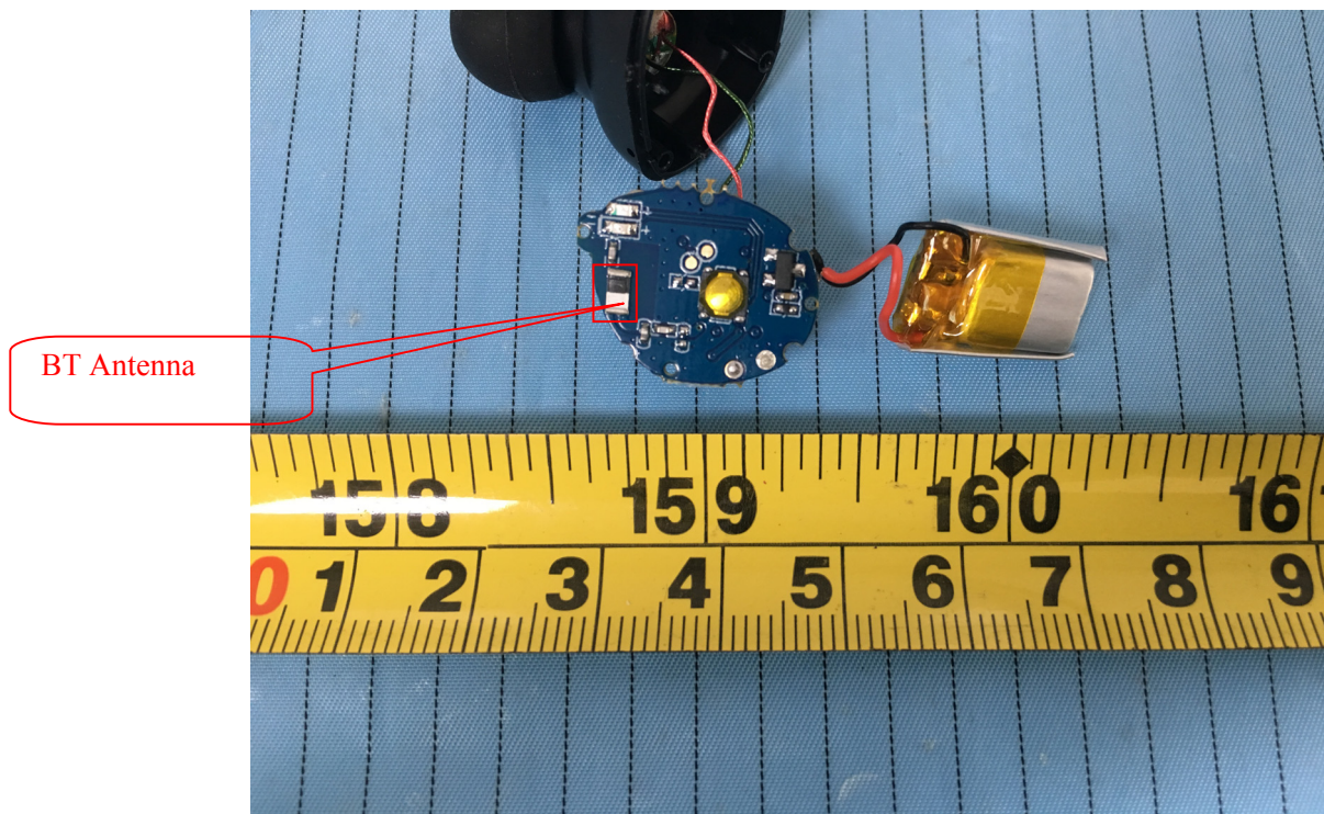
Charging Case:
