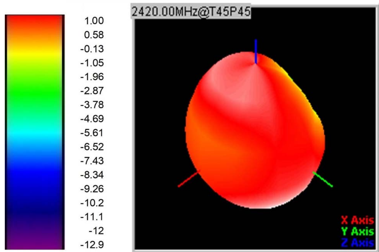
3D radiation pattern diagram (2420MHz)
