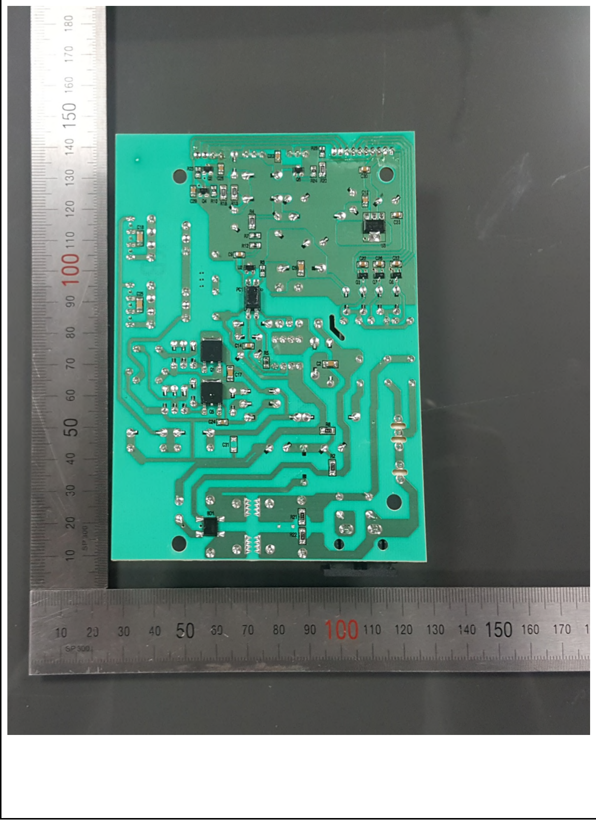
View of PCB(Bottom)
