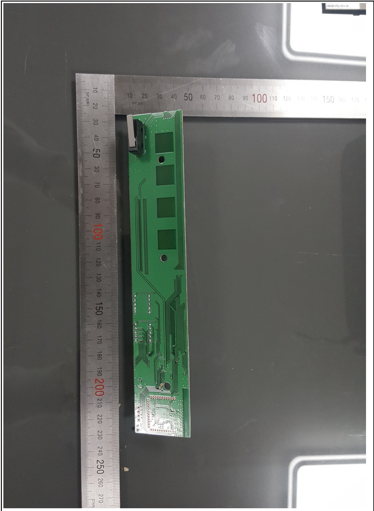
View of PCB2(Bottom)
