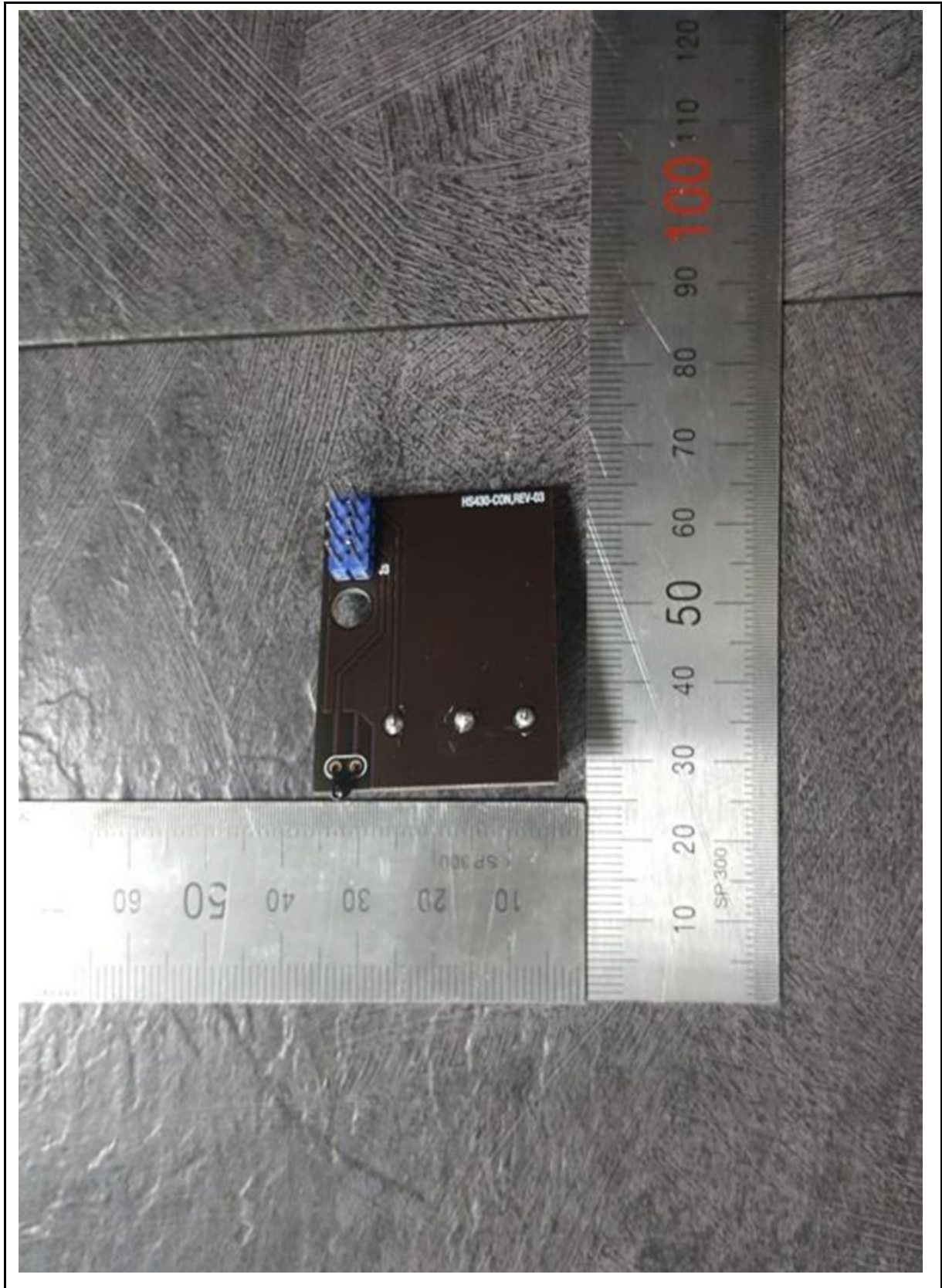
View of PCB3(Bottom)
