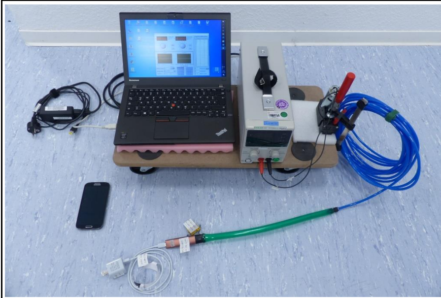
EUT VEEV + Auxillary equipment
