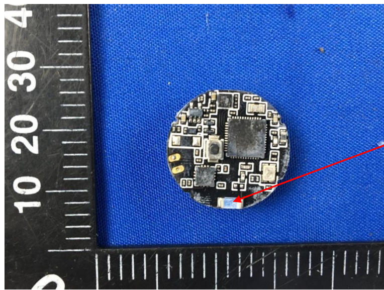
Bluetooth Antenna
