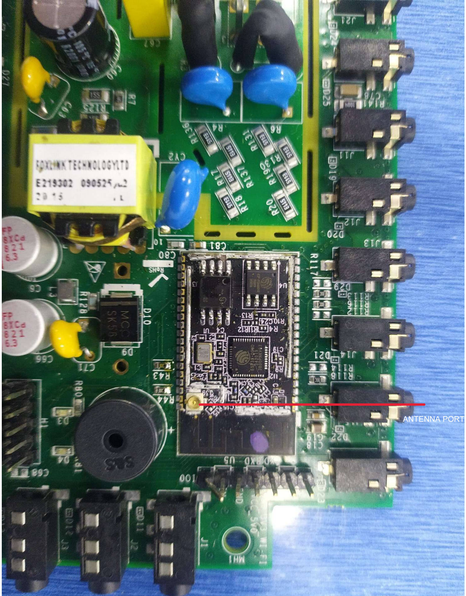
Photograph without Shielded Case and Antenna Port Location
